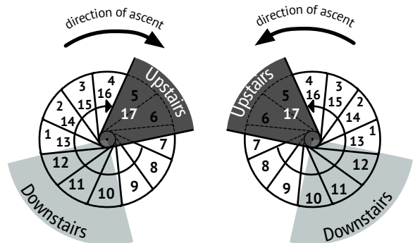
17 STEPS landing included (17 RISES) Height between floors: Min. 349 cm - Max. 408 cm
